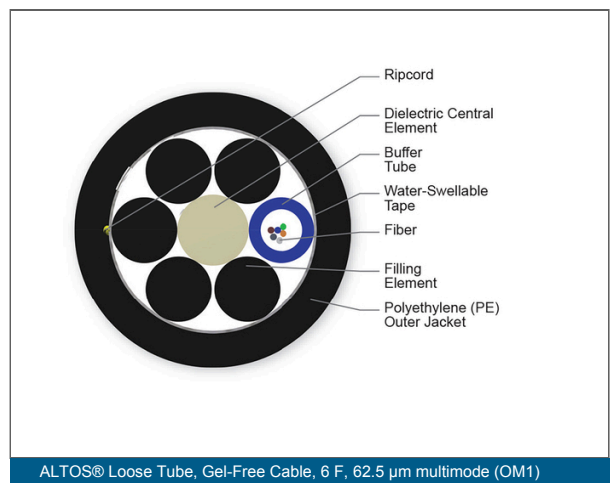
ALTOS® Loose Tube, Gel-Free Cable, 6 F, 62.5 µm multimode (OM1)
