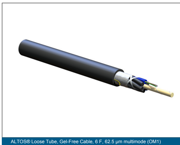
ALTOS® Loose Tube, Gel-Free Cable, 6 F, 62.5 µm multimode (OM1)
